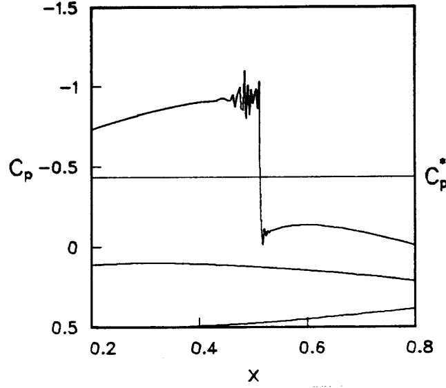
Figure 3: Coefficient of Pressure Showing Oscillations at Shock.
