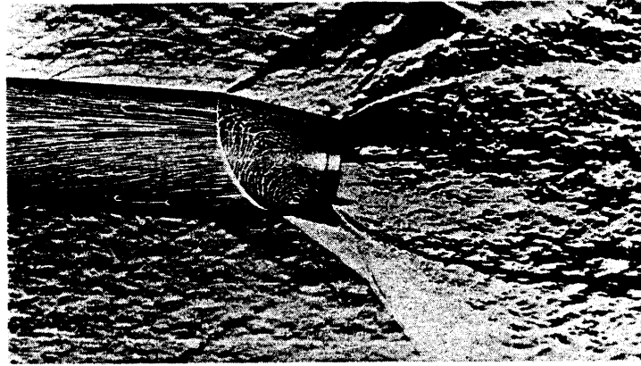
SIMULATION OF BOATTAIL AFTER BODY FLOW FIELD R = 2.9 \times 10^6 , M = 0.9 , \alpha = 6^\circ (DEIWERT, 1960)
