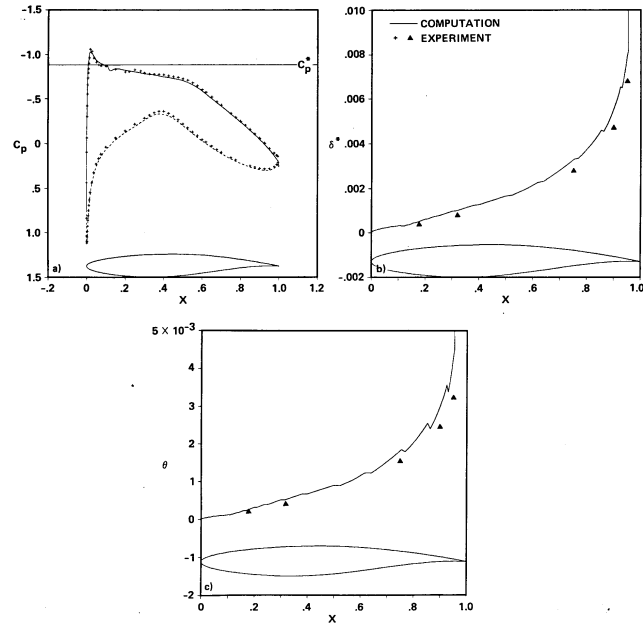
Figure 22: Viscous Results for RAE2822 Airfoil at Re = 5.7 \times 10^6 , M_\infty = 0.676 , \alpha = 1.93^\circ .
