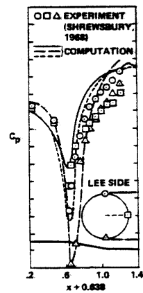
COMPARISON OF SURFACE PRESSURE DISTRIBUTION
