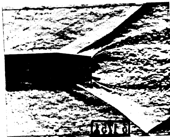
SCHLIEREN PHOTOGRAPH (Agrell, FFA)
