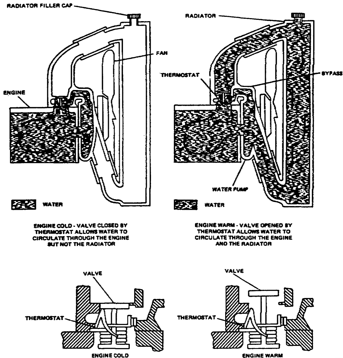
FIGURE 72. COOLANT BYPASS.
