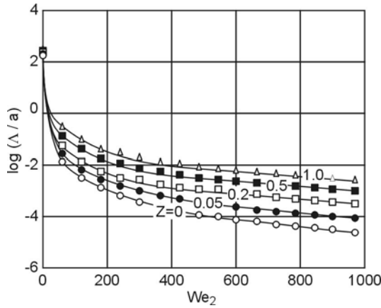
Fig. 4.26. Wavelength of the most unstable surface wave versus We_g as a function of Ohnesorge number Z [114].
