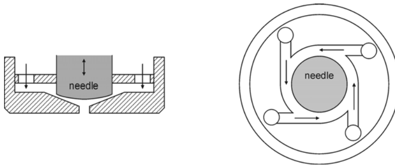
Fig. 4.18. Schematic illustration of the tangentially arranged swirl ports
