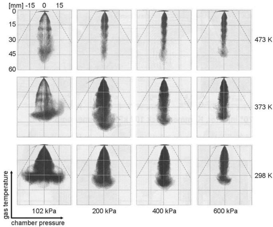
Fig. 2.20. Influence of ambient temperature on the spray structure (pressure-swirl atomizer) [14], pictures at 2 ms after energizing the injector, p_{rail} = 7 MPa
