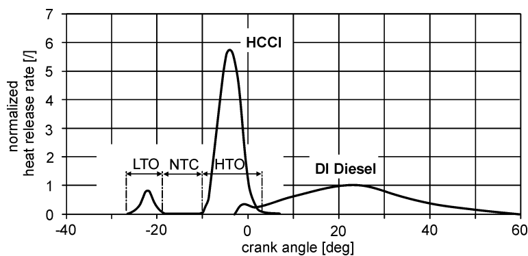
Fig. 6.27. Two-stage heat release of HCCI diesel combustion, schematic diagram
