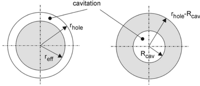
Fig. 4.8. Estimation of the artificial bubble size
