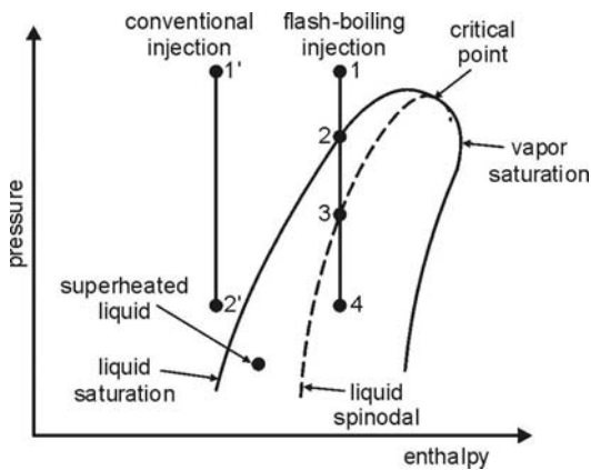
Fig. 4.48. Comparison of conventional injection and flash-boiling injection [99]
