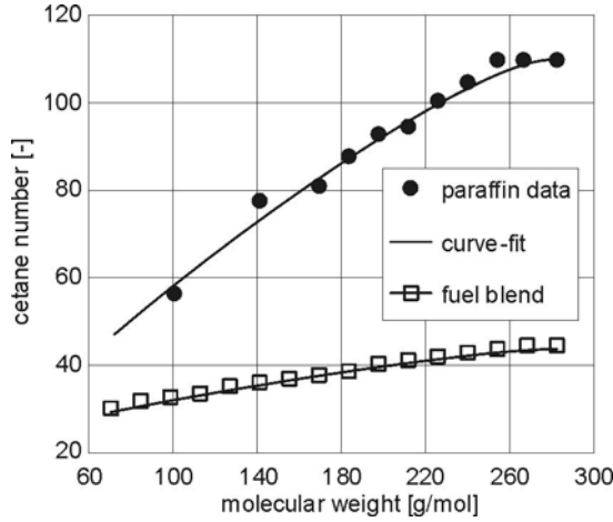
Fig. 4.57. Cetane number as function of molecular weight of paraffins (alkanes), data from [120]
