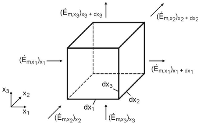
Fig. 3.8. Convective energy fluxes through a control volume
