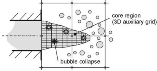
Fig. 4.10 Primary break-up model based on locally resolved break-up rates
