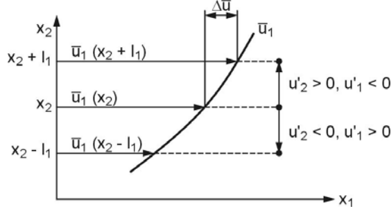
Fig. 3.10. Prandtl mixing-length model
