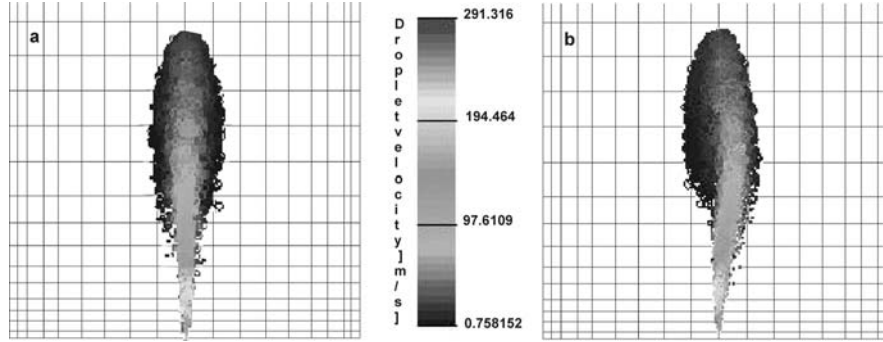
Fig. 4.11. Appearance of spray cone under perpendicular views and droplet velocities. a front view, b side view [143]
