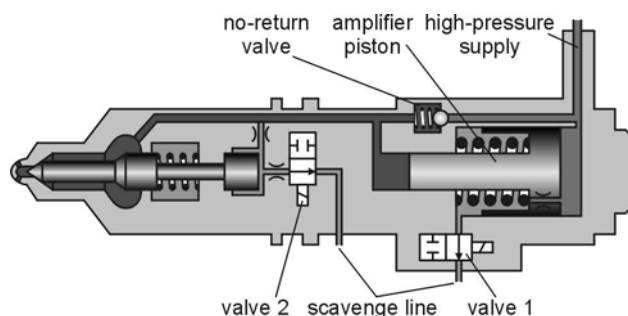
Fig. 6.12. Amplified pressure common-rail system from Bosch [14]
