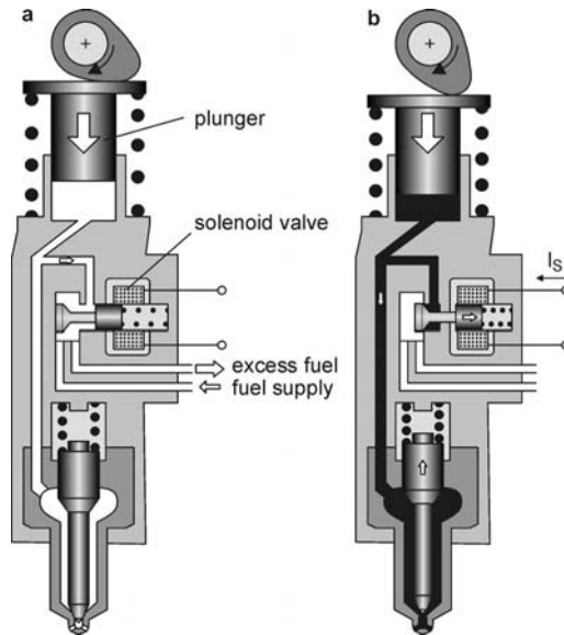
Fig. 2.28. Unit injector: schematic of injection control [46]
