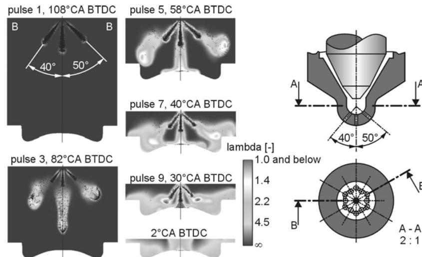
Fig. 6.33. Numerical investigation of mixture formation for early in-cylinder injection
