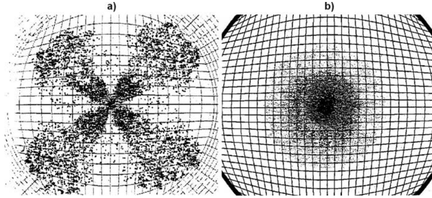
Fig. 5.7. Elimination of ninety-degree artifacts in Cartesian meshes. Both pictures show a hollow-cone spray directed towards the viewer [15]: a standard approach, b enhanced method
