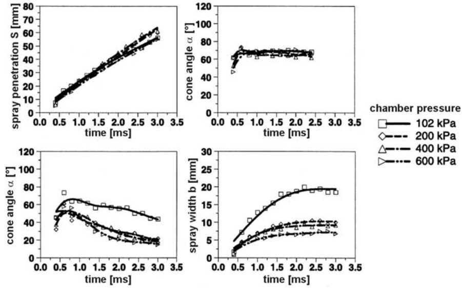
Fig. 2.19. Influence of ambient pressure and injection pressure on the spray structure (pressure-swirl atomizer) [14], T_{chamber} = 298 K, p_{rail} = 7 MPa, t = 0.0 ms: energizing of injector
