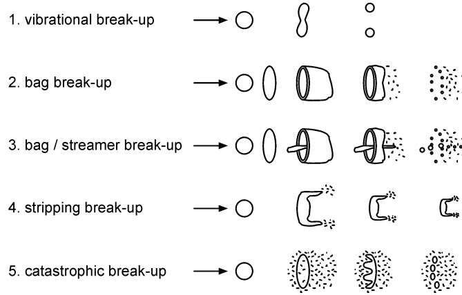
Fig. 2.5. Drop break-up regimes according to Wierzba [59]
