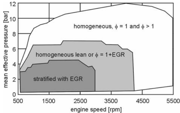
Fig. 6.18. GDI operating modes within the engine map [93]
