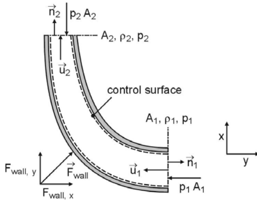
Fig. 3.3. Momentum equation: forces acting on a control volume
