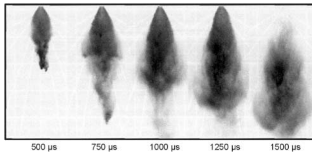
Fig. 2.15. Temporal development of a spray from a pressure-swirl atomizer [25], p_{rail} = 10 \text{ MPa} , p_{chamber} = 0.24 \text{ MPa} , T_{chamber} = 393 \text{ K}
