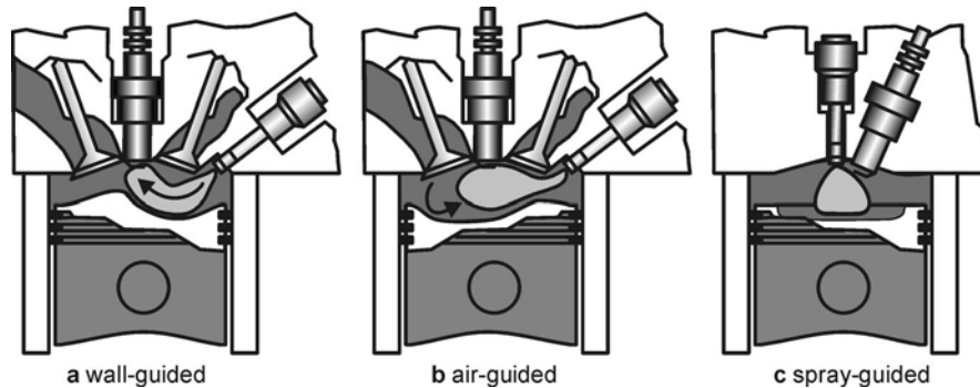
Fig. 6.19. Schematic description of the three possible stratified-charge combustion concepts
