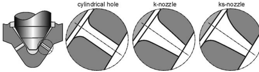
Fig. 2.32. Nozzle hole geometries
