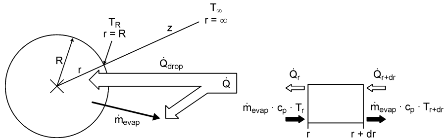
Fig. 4.37. Definition of coordinate system and heat fluxes
