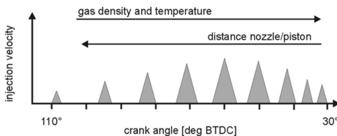
Fig. 6.31. Pulsed injection strategy for early in-cylinder injection
