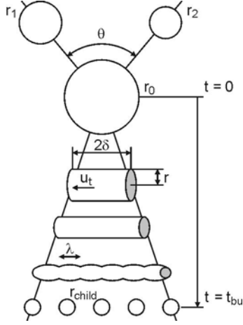
Fig. 4.59. Schematic representation of ligament formation and break-up [40]
