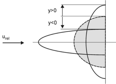
Fig. 4.21. ETAB model: an initial droplet deformation velocity results in an elongation of the drop in the direction of flight
