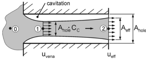
Fig. 4.3. One-dimensional cavitating nozzle hole flow
