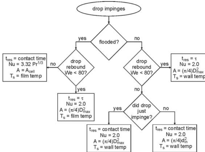
Fig. 4.69. Heat transfer model of Eckhause and Reitz [31]
