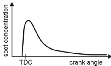
Fig. 6.3. Soot concentration as function of crank angle, schematic diagram
