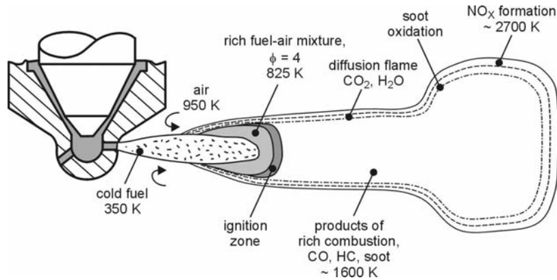
Fig. 6.2. Conventional diesel spray combustion and production of \text{NO}_x and soot (PM)
