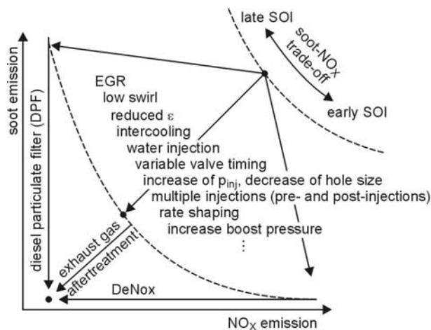
Fig. 6.4. Soot- \text{NO}_x trade-off: measures for reduction of soot and \text{NO}_x in engine emissions
