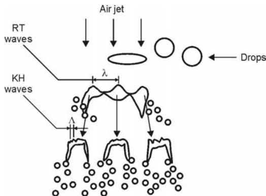
Fig. 4.28. Schematic diagram of break-up mechanisms in the catastrophic break-up regime [58]
