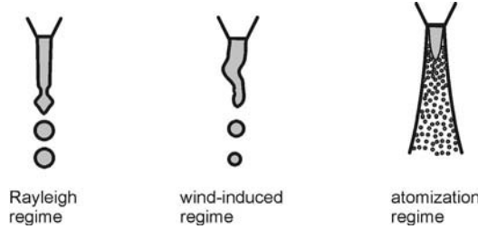
Fig. 2.3. Schematic description of jet break-up regimes
