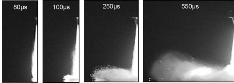
Fig. 2.23. Time evolution of an impinging spray, [1], p_{inj} = 120 MPa, p_{chamber} = 0.1 MPa ( N_2 ), d_{nozzle} = 0.18 mm, T_{wall} = 298 K
