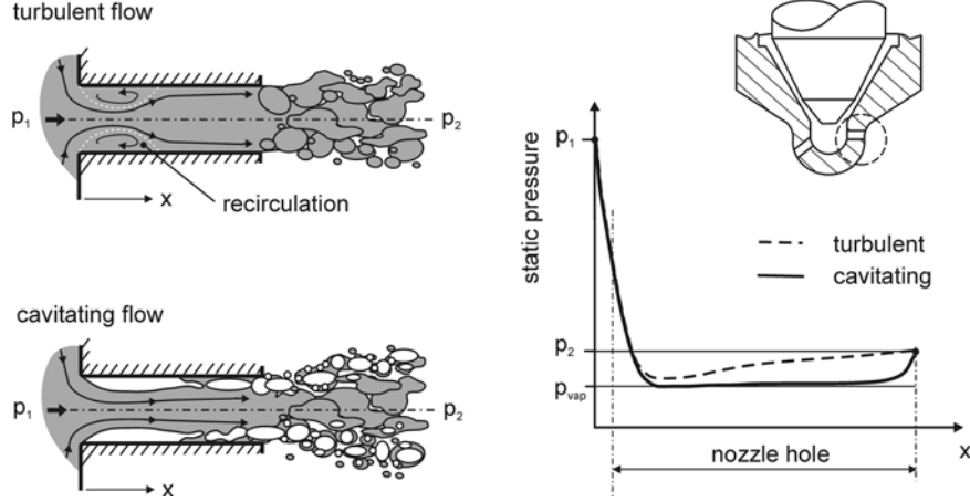
Fig. 2.12. Cavitating and non-cavitating nozzle hole flow
