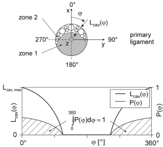
Fig. 4.13. 3D spray angle, example: asymmetric flow [14]
