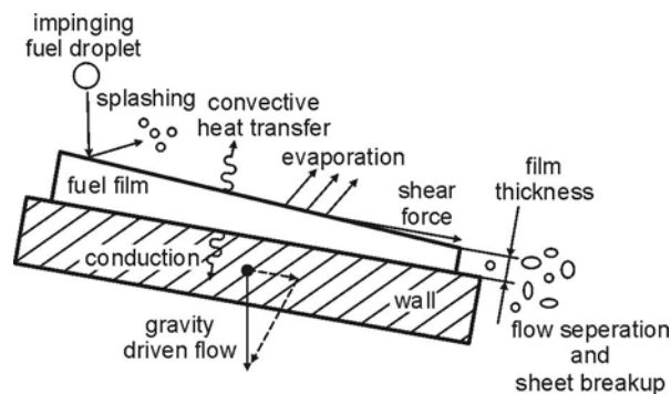
Fig. 4.68. The major physical phenomena governing film flow [133]
