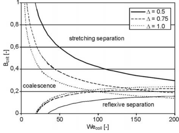
Fig. 4.57. Influence of droplet size ratio on the coalescence/stretching separation (Eq. 4.240) and on the coalescence/reflexive separation transition criterion (Eq. 4.245)
