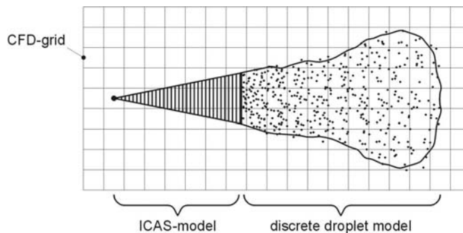
Fig. 5.11. Schematic illustration of the Interactive Cross-sectionally Averaged Spray (ICAS) method
