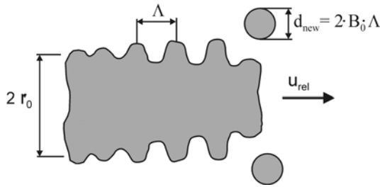
Fig. 4.24. Schematic illustration of the Kelvin-Helmholtz model
