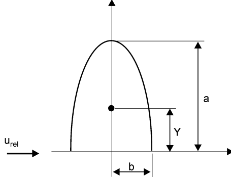
Fig. 4.23. Droplet deformation and breakup model (DDB model), schematic diagram of the deforming half drop
