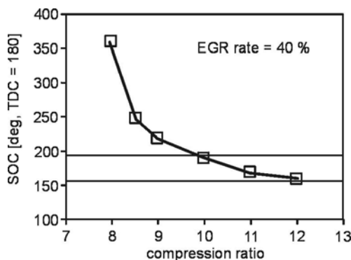
Fig. 6.36. Start of combustion versus compression ratio [71]
