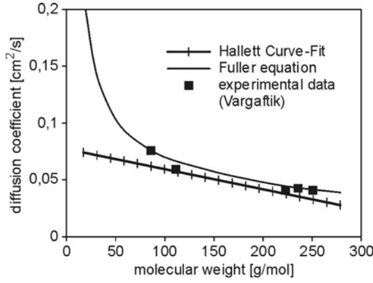
Fig. 4.42. Binary diffusion coefficients for alkanes and air [77]
