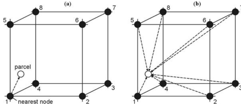
Fig. 5.5. Gas-droplet momentum exchange: a standard method, b enhanced approach
