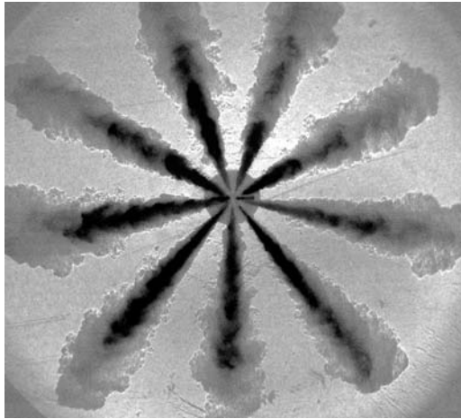
Fig. 2.8. Distribution of liquid (black) and vapor (gray) in an evaporating high-pressure diesel spray from a multi-hole nozzle under engine like conditions. Measurement technique: superposition of Schlieren technique (vapor and liquid) and Mie scattering (liquid)
