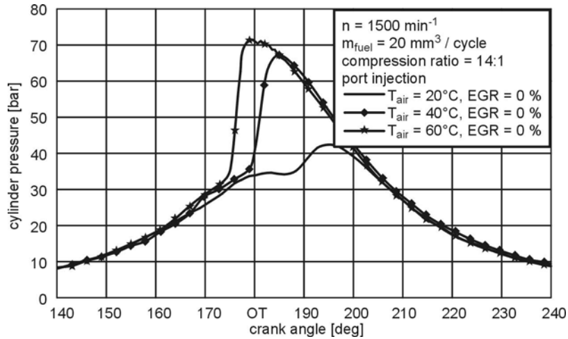
Fig. 6.41. Effect of inlet air temperature on HCCI combustion [94]
