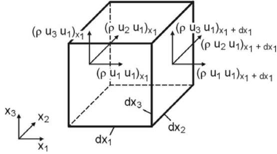
Fig. 3.6. Momentum fluxes entering and exiting the control volume
