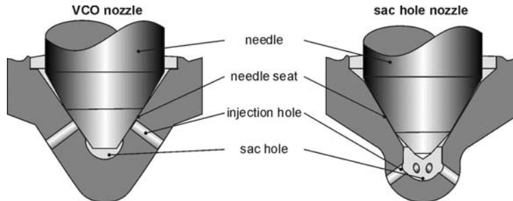
Fig. 2.31. Nozzle types
