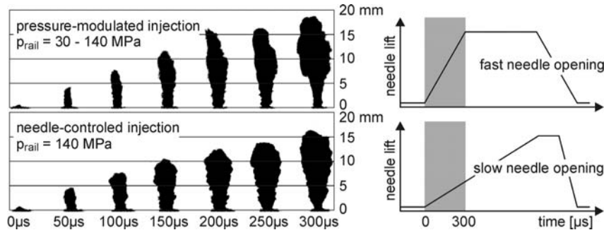
Fig. 6.14. Optical investigation of a ramp-type injection: comparison of pressure-modulated and needle lift controlled rate shaping during the first 300 \mu\text{s} of injection [80]
