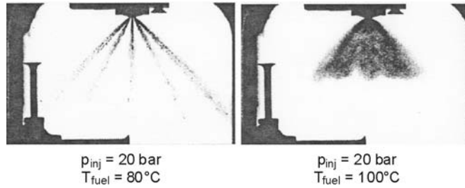
Fig. 4.49. Comparison of flashing and non-flashing full-cone sprays [98]
