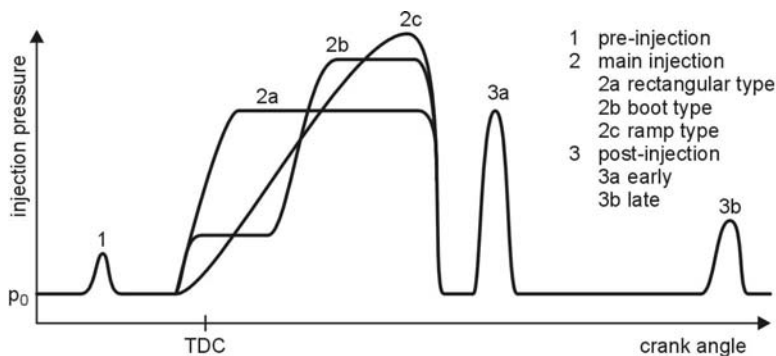
Fig. 6.5. Schematic diagram of a multiple injection
