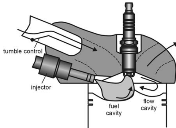
Fig. 6.21. Wall-air-guided technique, FSI combustion concept, Volkswagen [83]
