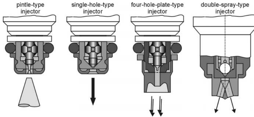
Fig. 2.35. Typical design of injectors, classified by the spray shape [34]
