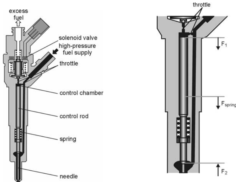
Fig. 2.26. A typical common rail injector [47]
