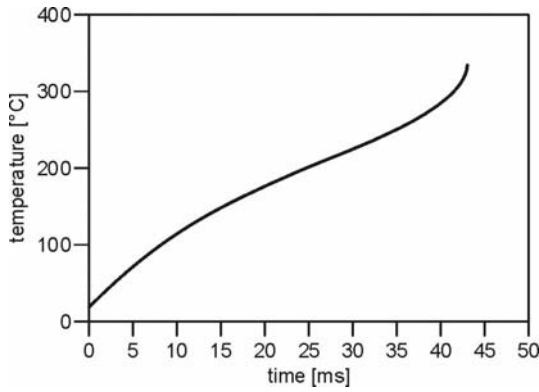
Fig. 4.43. Change of liquid temperature during evaporation of a multi-component diesel droplet (initial values: D = 100 \text{ }\mu\text{m} , u = 0 \text{ m/s} , T_{drop} = 300 \text{ K} , T_{gas} = 973 \text{ K} , p_{gas} = 0.1 \text{ MPa} ) [100]
