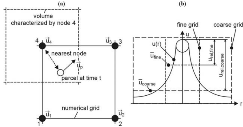
Fig. 5.1. Momentum exchange between liquid and gas phase
