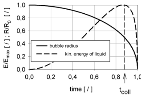
Fig. 4.14. Bubble radius and kinetic energy during collapse
