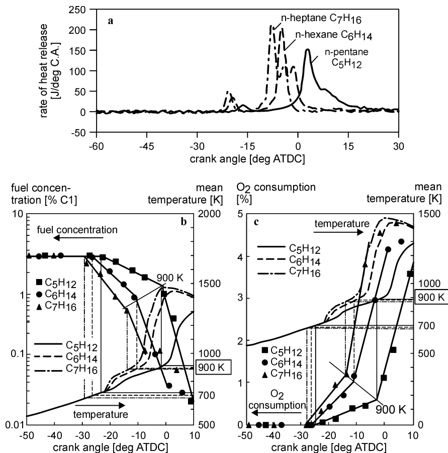
Fig. 6.42. Comparison of oxidation process for different single-component fuels (data from [92]). a rate of heat release, b fuel consumption, c O_2 consumption
