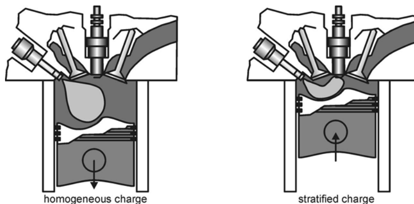
Fig. 6.16. Homogeneous (early injection) and stratified-charge mode (late injection)
