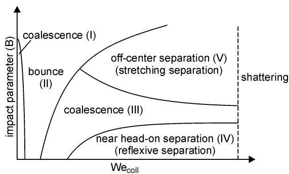
Fig. 4.55. Schematic of droplet collision regimes
