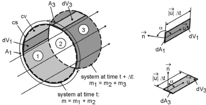
Fig. 3.1. System-to-control-volume transformation: system moving through a control volume, two-dimensional flow and control volume
