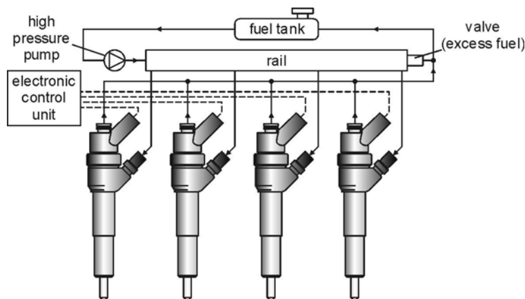
Fig. 2.25. The common rail injection system
