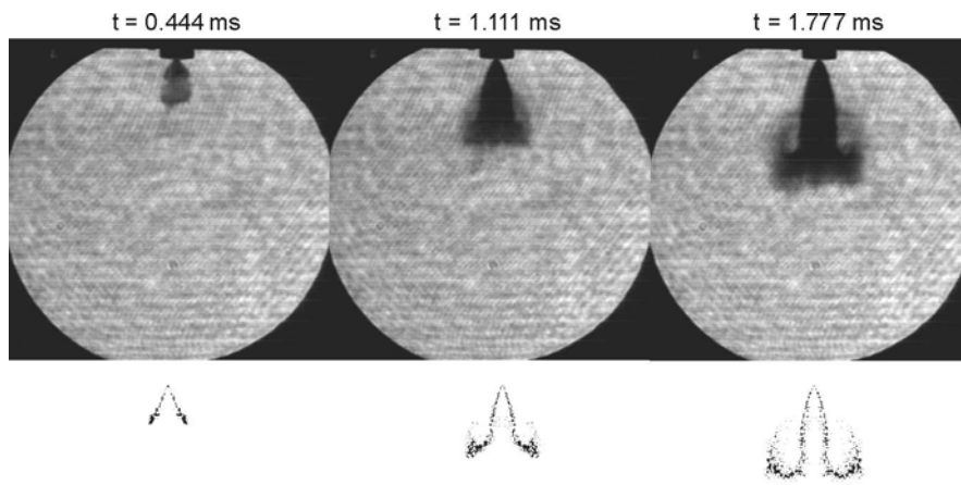
Fig. 4.33. Measured and calculated spray images, gas pressure: 366 kPa, [135]
