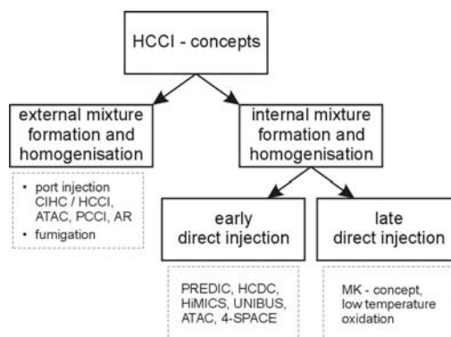
Fig. 6.30. Mixture formation concepts for HCCI-engines [56]
