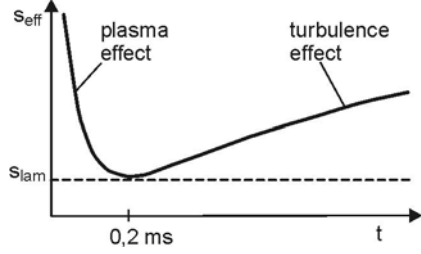
Fig. 4.75. Characteristic behavior of the effective flame speed after ignition [134]
