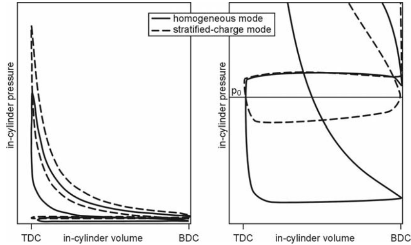
Fig. 6.17. Reduction of throttle losses, stratified-charge combustion
