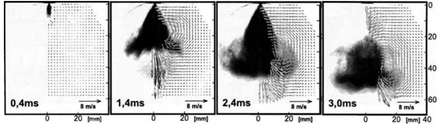
Fig. 2.16. Temporal development of the secondary gas flow around a spray from a pressure-swirl atomizer [14], p_{rail} = 7 \text{ MPa} , p_{chamber} = 0.102 \text{ MPa} , T_{chamber} = 298 \text{ K}
