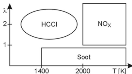
Fig. 6.24. HCCI-combustion: simultaneous reduction of soot and \text{NO}_x
