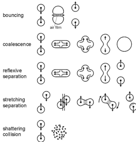
Fig. 4.56. Mechanisms of droplet collision
