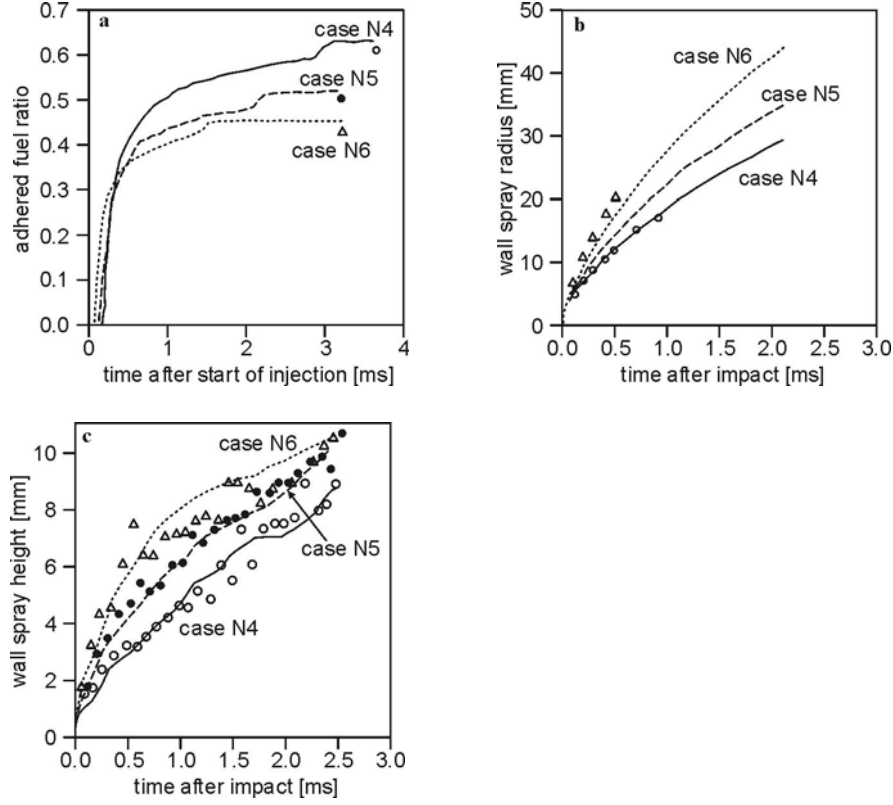
Fig. 4.67. a Measured and predicted adhered fuel ratio, b wall spray radius, c wall spray height, [11]
