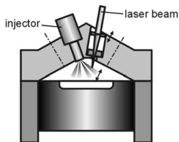
Fig. 6.23. Laser-induced ignition [25]
