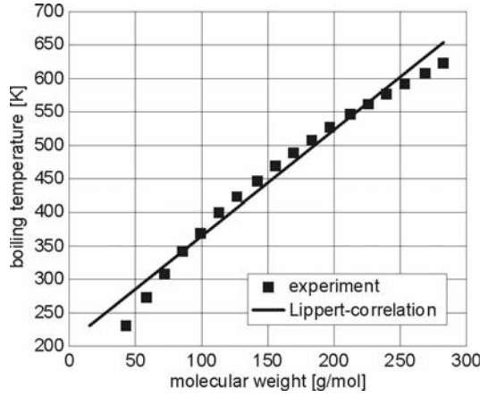
Fig. 4.41. Boiling temperature of alkanes as function of molecular weight
