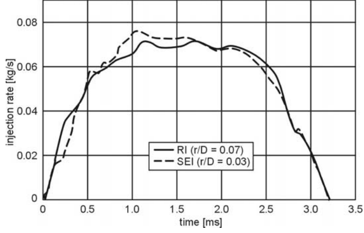
Fig. 4.4. Injection profiles for sharp-edged (SEI) and round-edged inlet (RI), [70]
