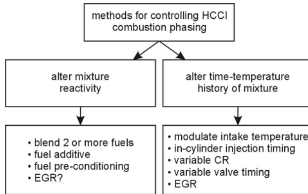
Fig. 6.35. Methods for controlling HCCI combustion phasing [87]
