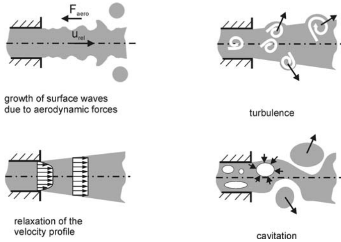
Fig. 2.9. Mechanisms of primary break-up
