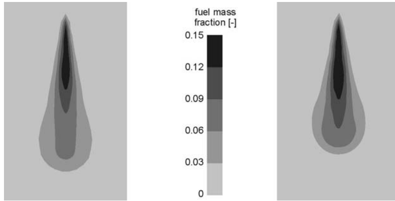
Fig. 4.45. Vapor phase fuel mass fractions for evaporating n\text{-C}_{14}\text{H}_{30} (left) and continuous multi-component fuel (right) sprays in nitrogen after 2 ms, m_{\text{fuel}} = 40 mg, T_{\text{fuel}} = 300 K, p_{\text{gas}} = 5.7 MPa, T_{\text{gas}} = 800 K, p_{\text{inj}} = 110 MPa [100]
