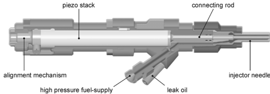
Fig. 6.10. Piezo injector with direct needle control [54]
