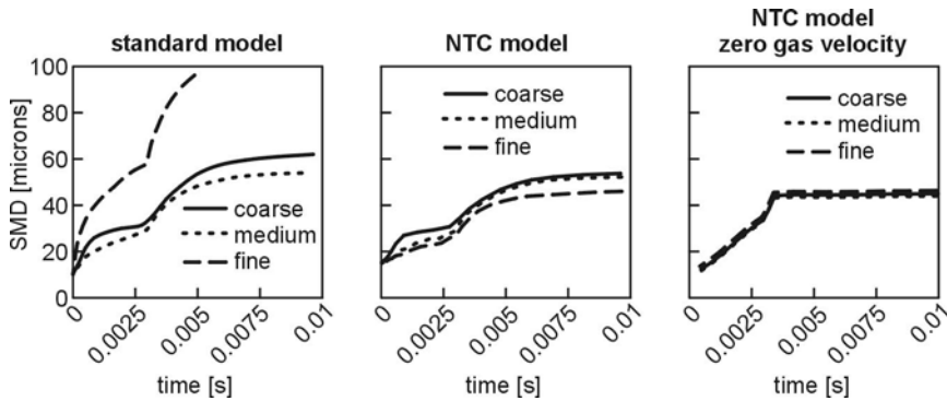
Fig. 5.10. Mesh dependency of standard and NTC collision model [15], diesel-type spray, Cartesian mesh
