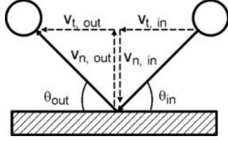
Fig. 4.65. Velocity components and respective angles for an impinging drop
