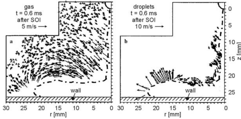
Fig. 2.22. a Typical flow field around an impinging full-cone spray, b droplet velocities [35], p_{inj} = 100 MPa, p_{chamber} = 1.0 MPa ( N_2 ), d_{nozzle} = 0.25 mm, T_{wall} = 298 K
