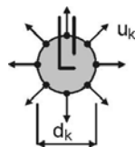
Fig. 4.74. Ignition kernel growth
