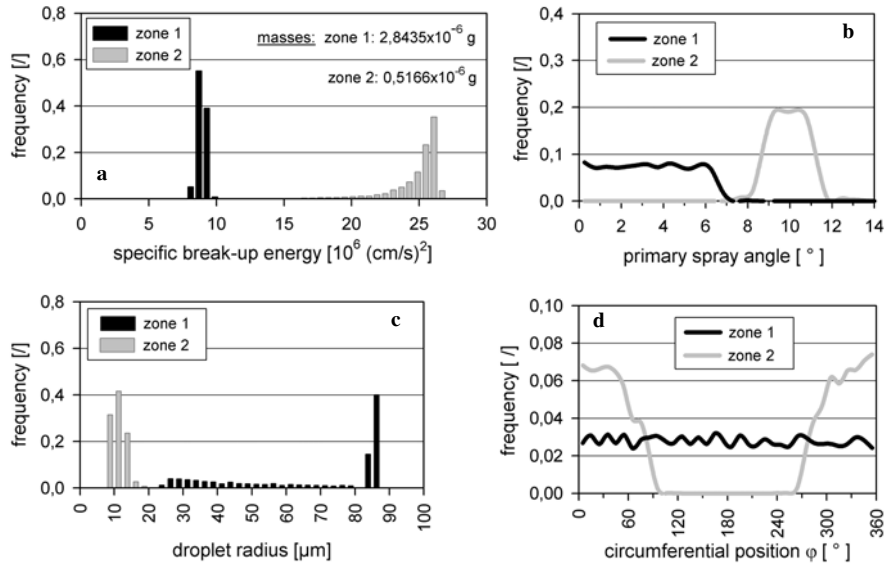
Fig. 4.15. Statistical analysis of relevant parameters during primary break-up [12]
