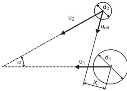
Fig. 4.54. Schematic illustration of geometric collision parameters
