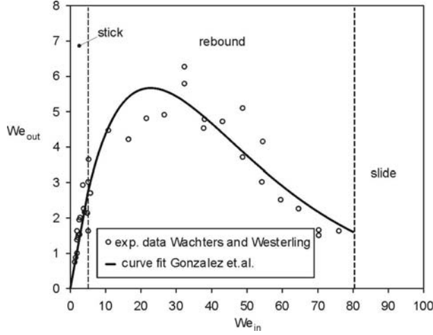
Fig. 4.63. Weber numbers of drops before and after impingement, data from [144]
