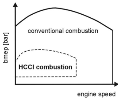
Fig. 6.26. Dual-mode operation
