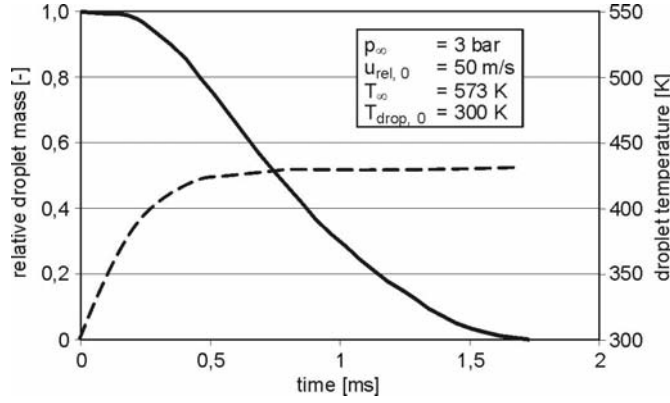
Fig. 4.38. Temperature and mass histories of an evaporating decane droplet
