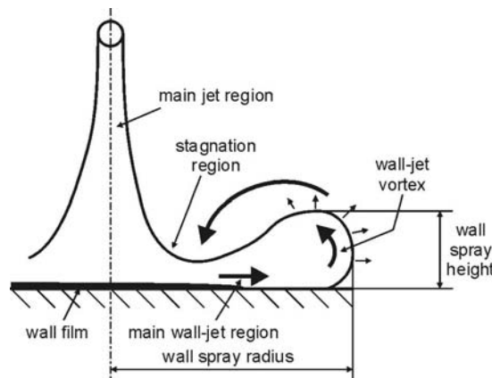
Fig. 2.21. Schematic illustration of an impinging full-cone spray
