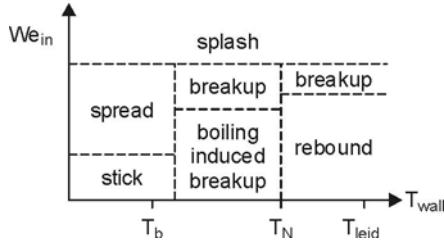
Fig. 4.62. Droplet impingement regimes and transition conditions for a dry wall [11]
