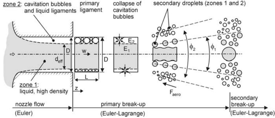
Fig. 4.12. Primary break-up model of Baumgarten et al. [13, 14]
