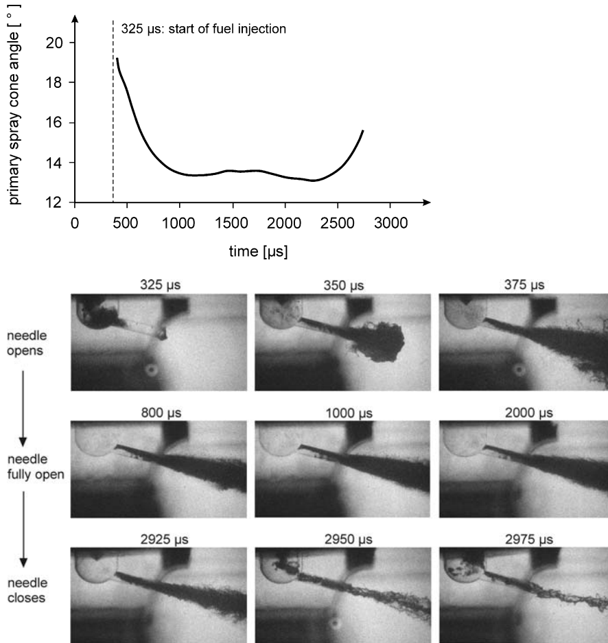
Fig. 2.13. Spray formation during injection. Data from [7], CR injector, p_{rail} = 60 MPa, p_{back} = 0.1 MPa, T_{air} = 293 K
