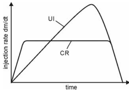
Fig. 2.29. Typical injection rate profiles of common rail and unit injector system
