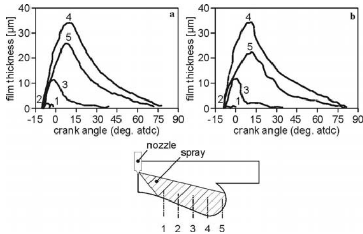
Fig. 4.72. Comparison of film thickness. a simulation, b measurement, data from [133]
