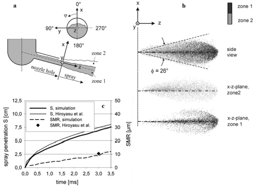
Fig. 4.16. Influence of the new primary break-up model on the dilute spray [12]
