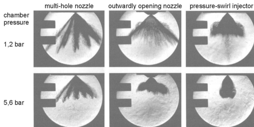
Fig. 2.37. Effect of injection pressure on the spray structure [26], p_{\text{rail}} = 10 \text{ MPa}
