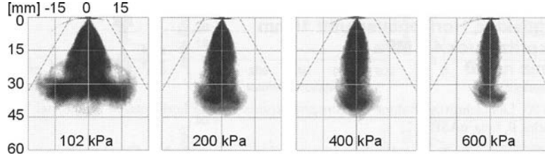
Fig. 2.18. Influence of ambient pressure on the spray structure (pressure-swirl atomizer) [14], pictures at 2 ms after energizing the injector, T_{chamber} = 298 K, p_{rail} = 7 MPa
