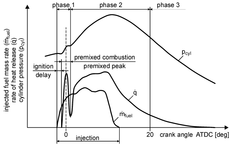
Fig. 6.1. Phases of the conventional diesel combustion process
