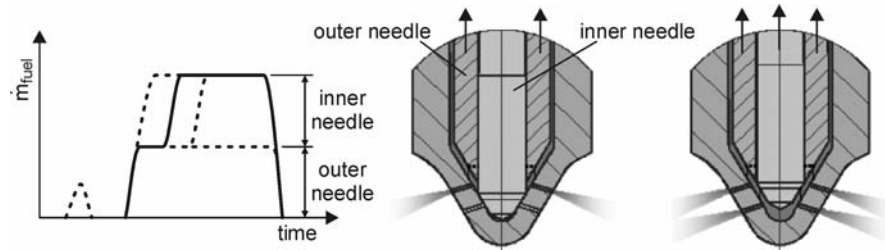
Fig. 6.11. Variable nozzle concept: possibility of rate shaping [9]
