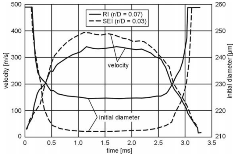
Fig. 4.5. Dynamic calculation of blob diameter and injection velocity, data from [70]
