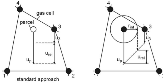
Fig. 5.9. Enhanced gas-drop momentum exchange: calculation of a representative gas velocity [3]
