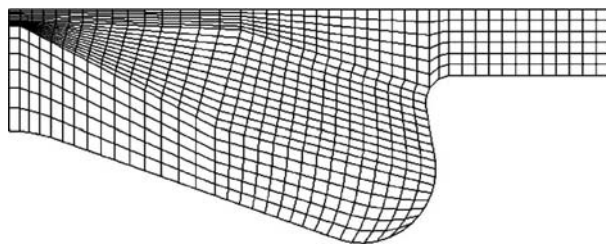
Fig. 5.4. Spray adapted grid for a DI diesel engine
