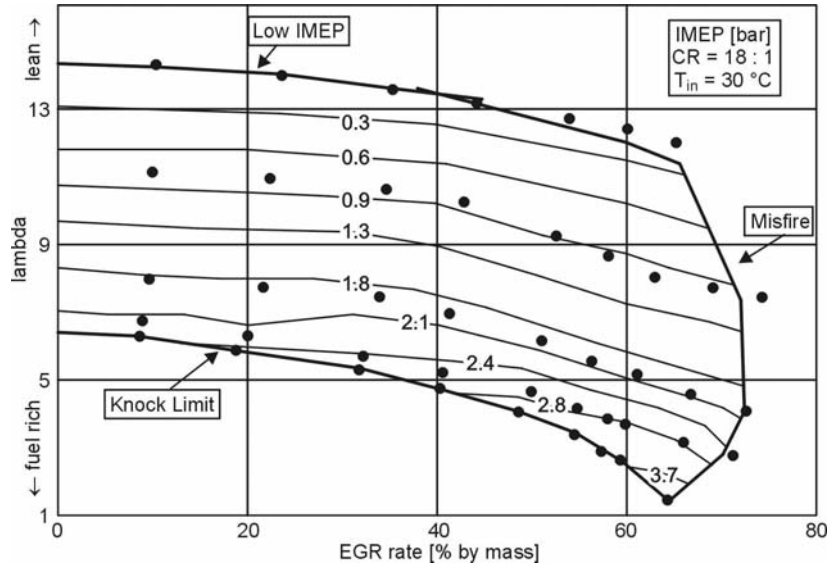
Fig. 6.39. Successful HCCI operational range and IMEP map. Parameter: IMEP, compression ratio 18:1, intake temperature 30°C, n-heptane [65]
