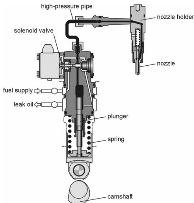
Fig. 2.30. Unit pump system [58]
