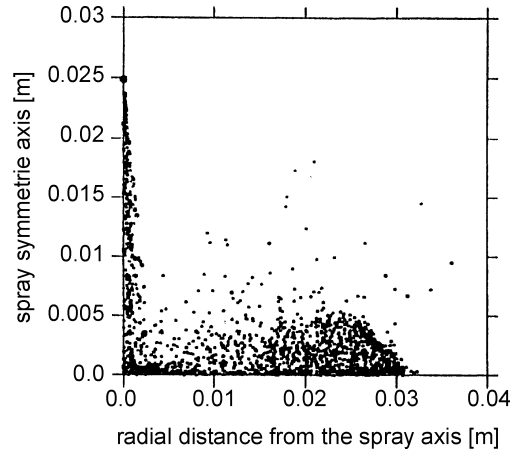
Fig. 4.66. Simulation of an impinging spray [11], t = 2 ms after SOI, atmospheric conditions
