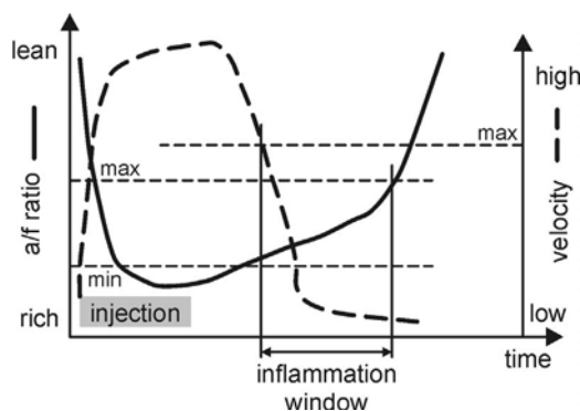
Fig. 6.22. Inflammation conditions in the spark gap [100]
