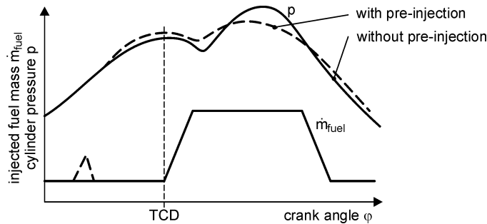
Fig. 6.6. Reduction of the premixed peak using a pre-injection, schematic diagram
