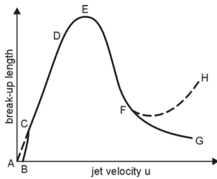
Fig. 2.4. Jet surface break-up length as function of jet velocity u [44]. ABC: Drip flow, CD: Rayleigh break-up, EF: first wind-induced break-up, FG (FH): second wind-induced break-up, beyond G (H): atomization regime
