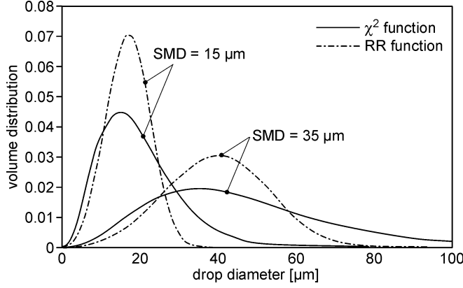
Fig. 4.6. Comparison of the Rosin-Rammler (RR) and \chi^2 size distributions [49]
