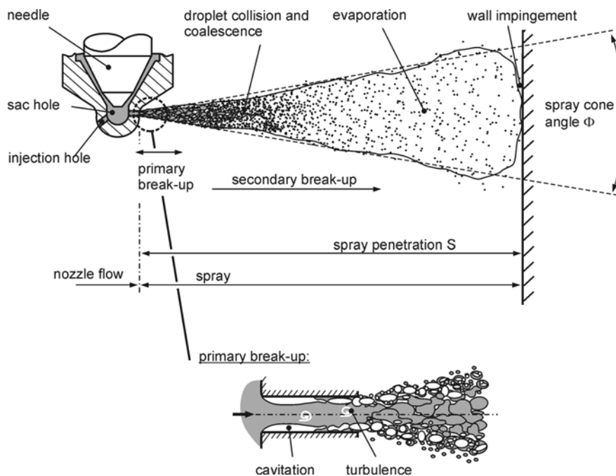
Fig. 2.6. Break-up of a full-cone diesel spray
