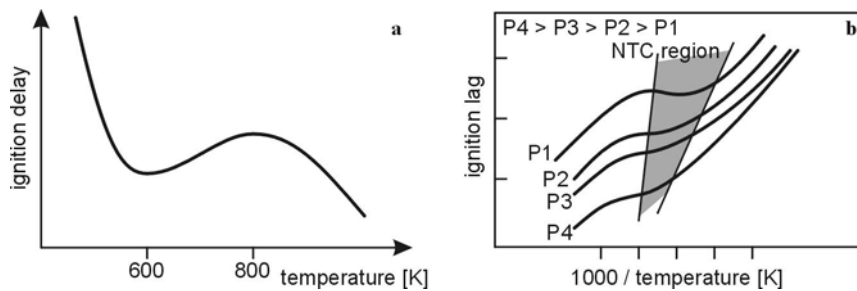
Fig. 6.28. Negative temperature coefficient for hydrocarbon ignition. a [84], b [103]
