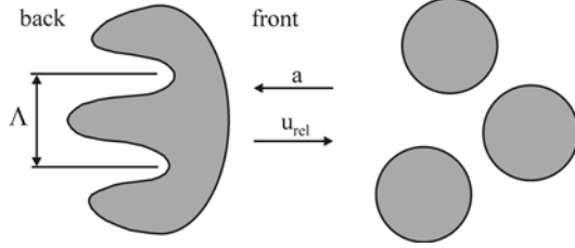
Fig. 4.27. Rayleigh-Taylor instability on a liquid drop
