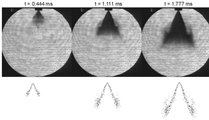
Fig. 4.32. Measured and calculated spray images, gas pressure: 101 kPa, [135]
