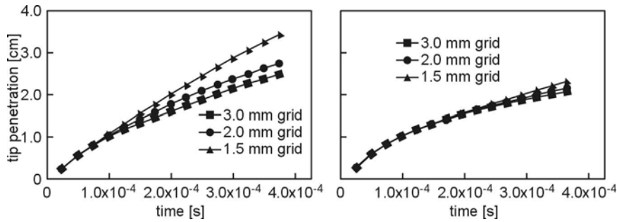
Fig. 5.6. Reduction of grid dependency due to an advanced modeling of momentum exchange between gas and liquid [5]
