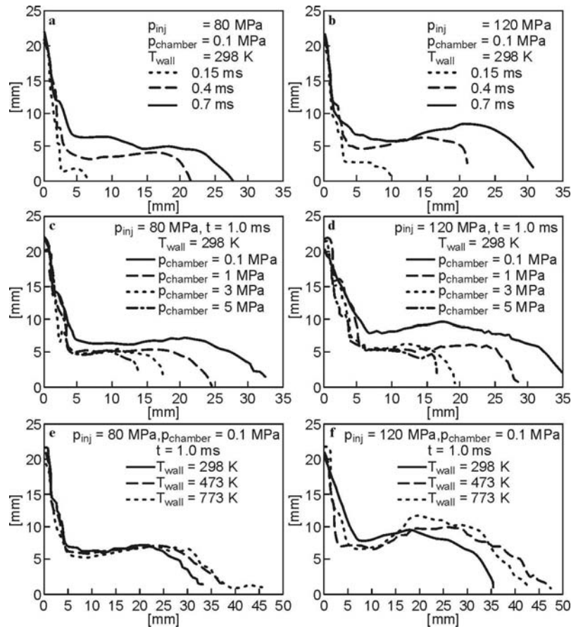
Fig. 2.24. Effect of injection pressure, chamber pressure and wall temperature on wall-spray impingement, data from [1], p_{inj} : 80 MPa and 120 MPa, chamber gas: N_2 , d_{nozzle} = 0.18 mm
