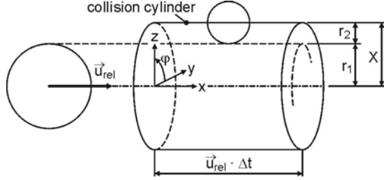
Fig. 4.60. Collision cylinder volume
