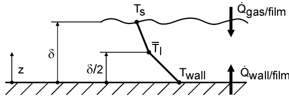
Fig. 4.51. Piecewise linear film temperature profile
