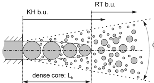
Fig. 4.29. Combined blob-HK/RT model
