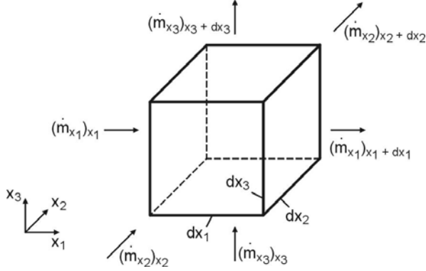
Fig. 3.5. Mass fluxes entering and exiting the control volume
