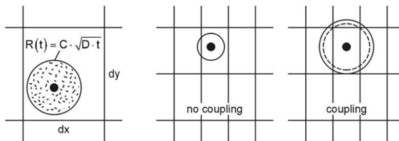
Fig. 5.8. Limitation of numerical diffusion: sub-grid scale vapor and momentum diffusion model [7, 3]
