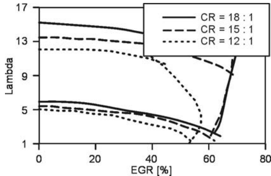
Fig. 6.40. Effect of compression ratio on the operational range of HCCI diesel combustion [17]
