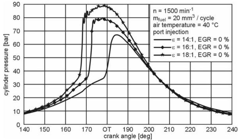
Fig. 6.37. Effect compression ratio on HCCI combustion [94]
