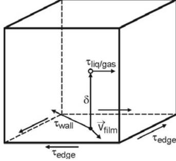
Fig. 4.71. Momentum cell
