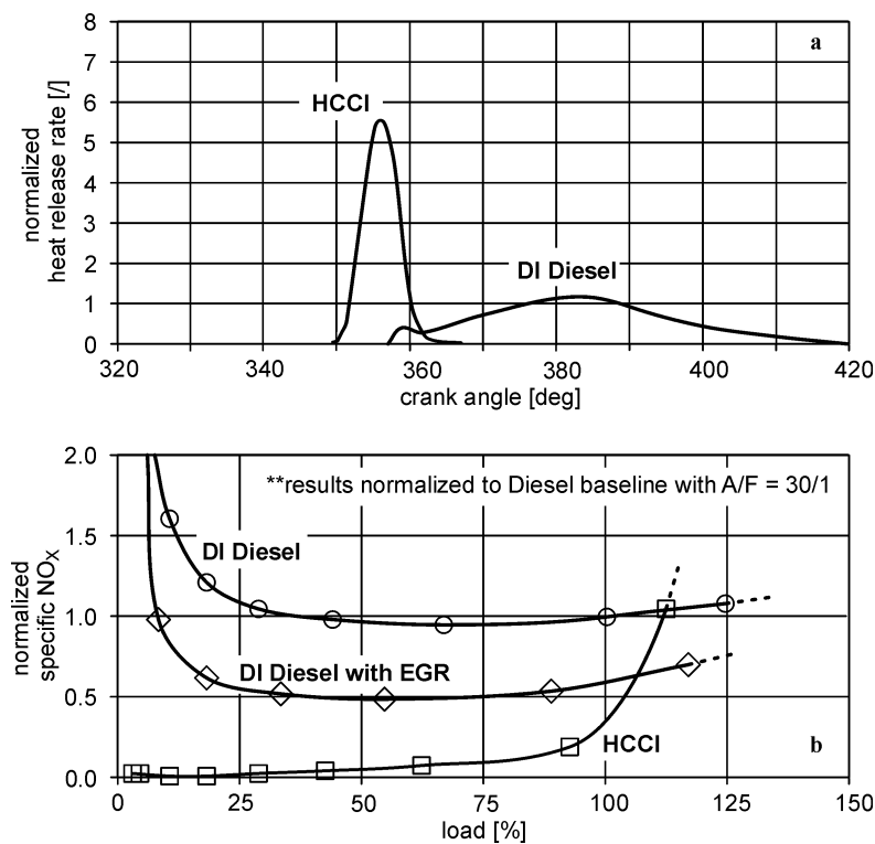
Fig. 6.29. Predicted \text{NO}_x emissions versus engine load for typical HCCI and DI-diesel combustion [87]. a assumed heat release, b \text{NO}_x emissions versus load, A/F: air-fuel ratio.
