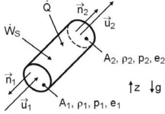
Fig. 3.4. One-dimensional pipe flow with heat and work
