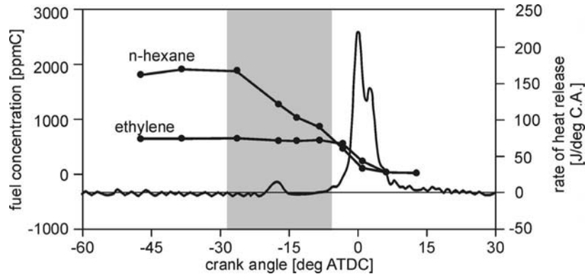
Fig. 6.43. Comparison of oxidation process for different fuels (data from [92])
