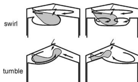
Fig. 6.20. Possible combustion chamber geometries as well as in-cylinder air motions, air-guided technique
