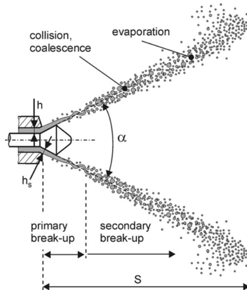
Fig. 2.14. Hollow-cone spray. Example: outwardly opening nozzle
