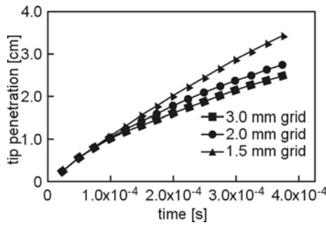
Fig. 5.2. Effect of grid resolution on spray penetration [5]
