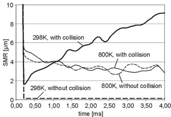
Fig. 4.58. Effect of the collision model on the SMR of an evaporating and a non-evaporating diesel spray
