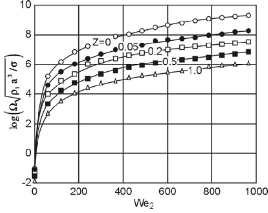
Fig. 4.25. Growth rate of the most unstable surface wave versus We_g as a function of Ohnesorge number Z [114].
