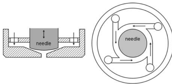
Fig. 2.38. Example of a high-pressure swirl atomizer with tangentially arranged swirl ports
