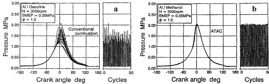
Fig. 6.25. Comparison of cylinder pressure histories. a SI operation (gasoline), b HCCI operation (labeled ATAC) with methanol [37]
