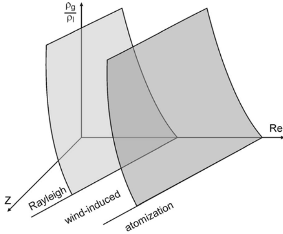
Fig. 2.2. Schematic diagram including the effect of gas density on jet break-up
