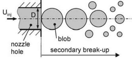
Fig. 4.1. Blob-method
