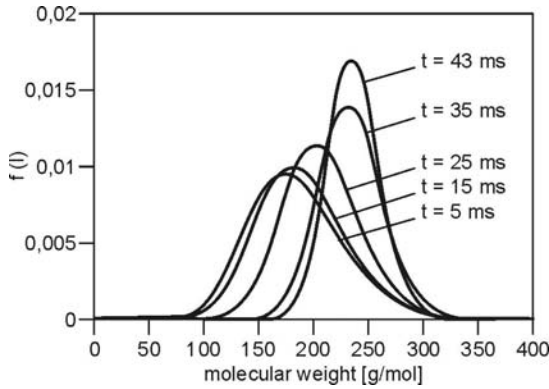
Fig. 4.44. Change of liquid composition during evaporation of a multi-component diesel droplet (initial values: D = 100 \text{ }\mu\text{m} , u = 0 \text{ m/s} , T_{drop} = 300 \text{ K} , T_{gas} = 973 \text{ K} , p_{gas} = 0.1 \text{ MPa} ) [100]
