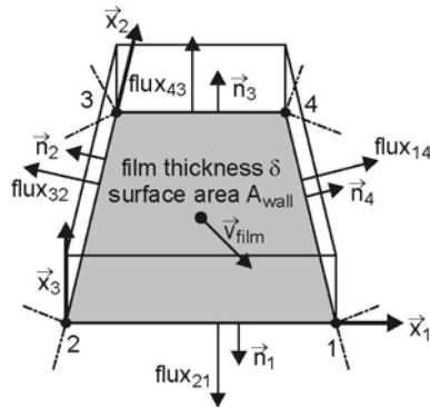
Fig. 4.70. Wall film cell and local coordinate system of the film model
