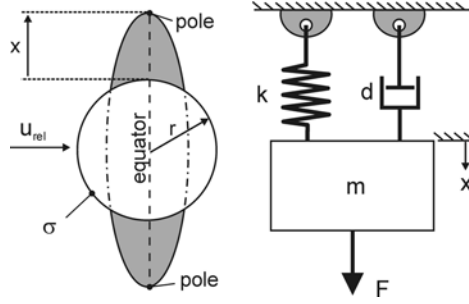
Fig. 4.20. Taylor-Analogy break-up model
