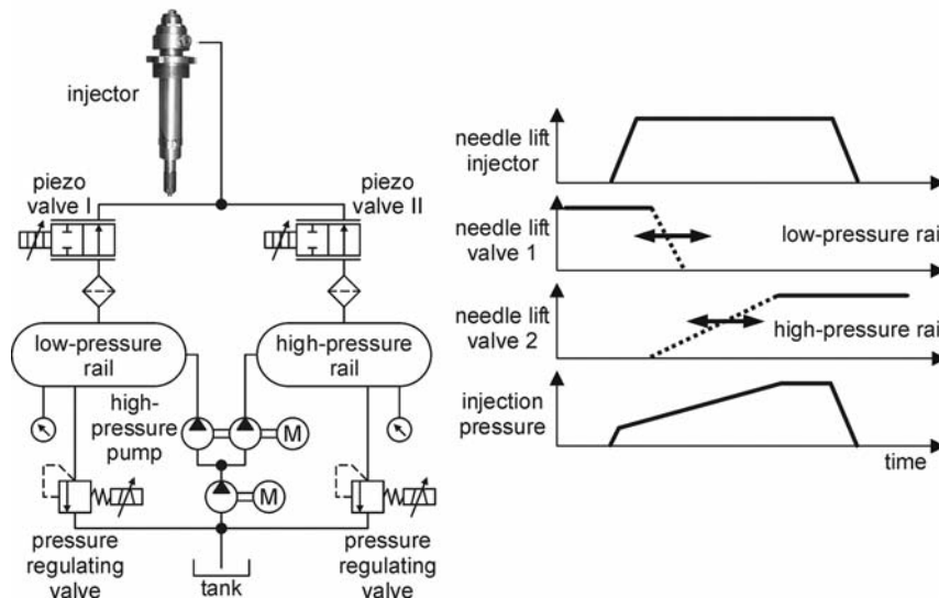
Fig. 6.13. Twin-CR system [50, 75]
