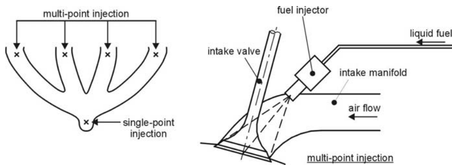
Fig. 2.33. Single-point and multi-point injection system
