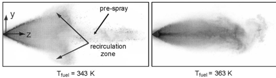
Fig. 4.50. Comparison of flashing and non-flashing hollow-cone sprays [126]
