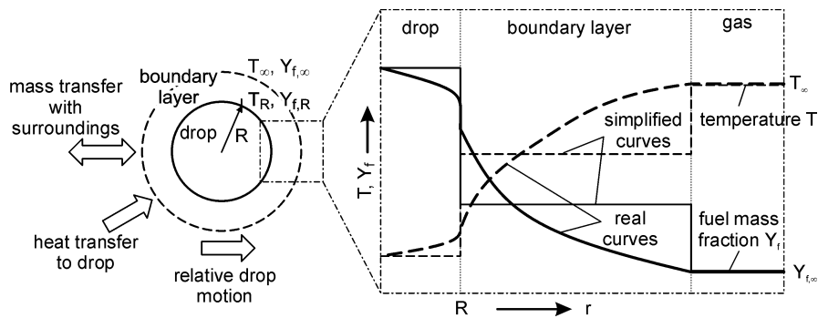
Fig. 4.36. Schematic view of drop vaporization
