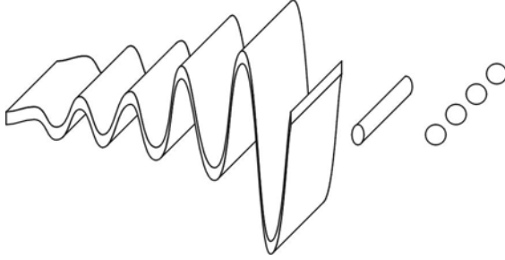
Fig. 4.19. Break-up of the liquid sheet into ligaments and droplets
