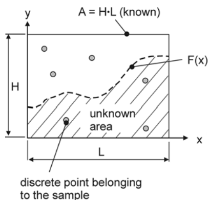
Fig. 3.12. Basic idea of the Monte-Carlo Method
