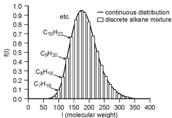
Fig. 4.39. Continuous and discrete representation of multi-component fuels
