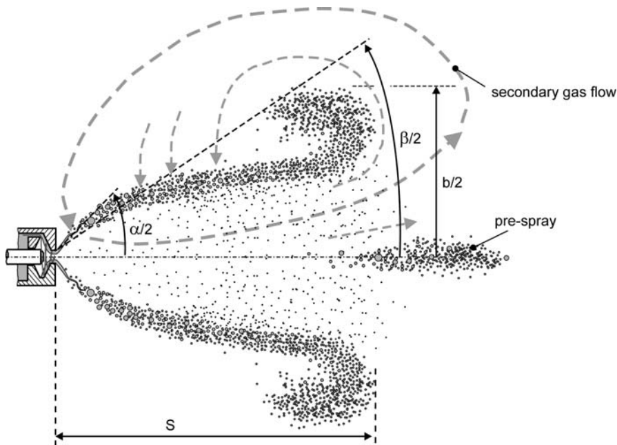
Fig. 2.17. Typical spray from a pressure-swirl atomizer (schematic illustration)
