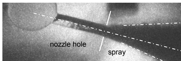
Fig. 2.11. Effect of an asymmetric distribution of cavitation inside the nozzle holes on the primary spray [36], p_{rail} : 60 MPa, p_{chamber} : 5 MPa, shadowgraphy
