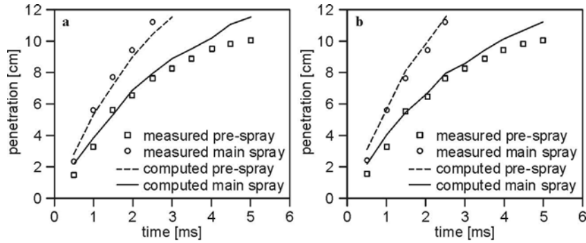
Fig. 4.31. Measured and predicted penetration. a case 1, b case 2 [125]
