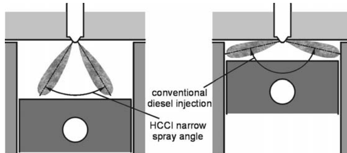
Fig. 6.32. Adaptation of spray angle for early in-cylinder injection
