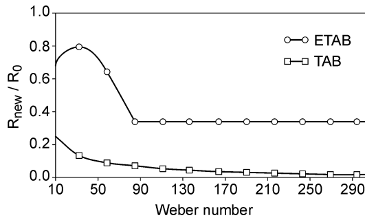
Fig. 4.22. Ratio of product and parent drop radii for the ETAB and the standard TAB model
