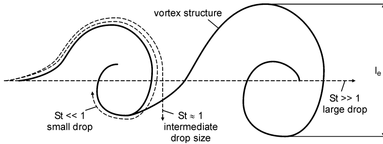
Fig. 4.53. Possible drop trajectories in a turbulent flow field [27]
