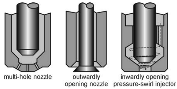
Fig. 2.36. Direct injection of gasoline: injector geometries [14]
