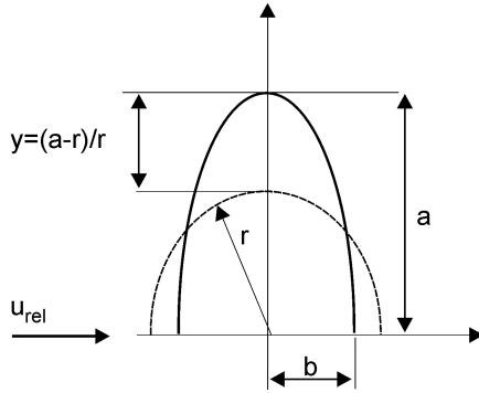
Fig. 4.35. Schematic diagram of the deforming half drop (DDB model)
