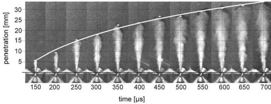
Fig. 2.7. Spray development during injection [53], p_{rail} = 70 MPa, p_{back} = 5 MPa, T_{air} = 890 K
