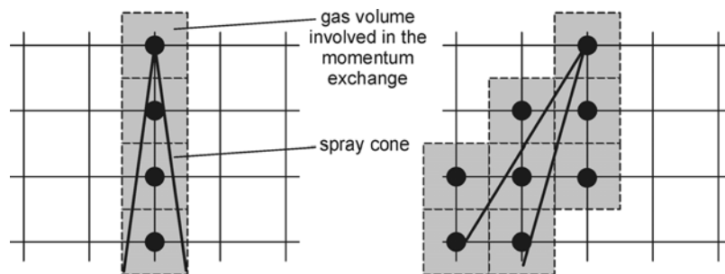
Fig. 5.3. Effect of grid orientation on spray penetration
