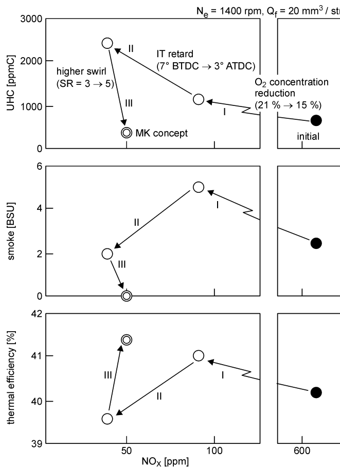
Fig. 6.34. Effects of EGR, retarded injection timing (IT) and increased swirl on exhaust emissions and thermal efficiency, Nissan MK-concept [43]
