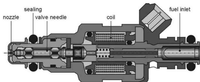
Fig. 2.34. Solenoid injector [34]
