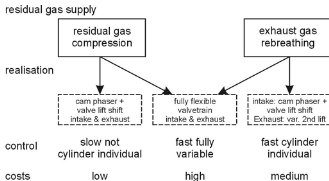
Fig. 6.38. Internal EGR: residual gas supply for HCCI operation [23]
