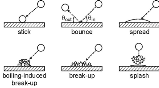
Fig. 4.61. Schematic illustration of different impact regimes [11]
