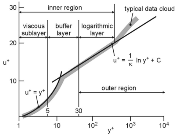
Fig. 3.11. Law of the wall: velocity profile in a turbulent boundary layer [12]
