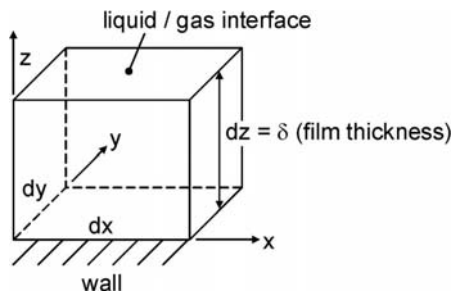
Fig. 4.52. Liquid film element and coordinate system
