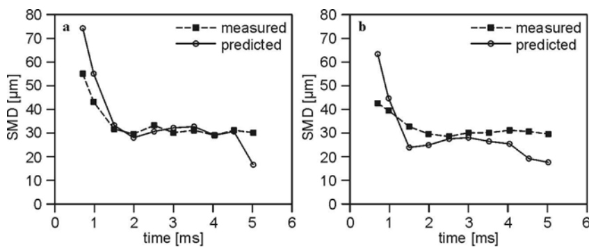
Fig. 4.30. Measured and predicted SMD. a case 1, b case 2, drop sizes averaged over a plane 39 mm downstream of the injector [125]
