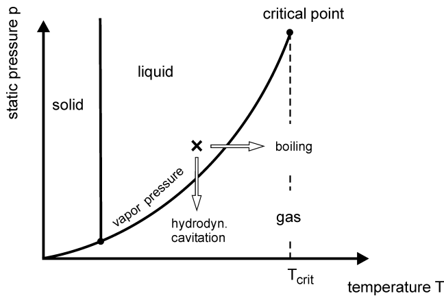
Fig. 2.10. Hydrodynamic cavitation, example: a single-component liquid
