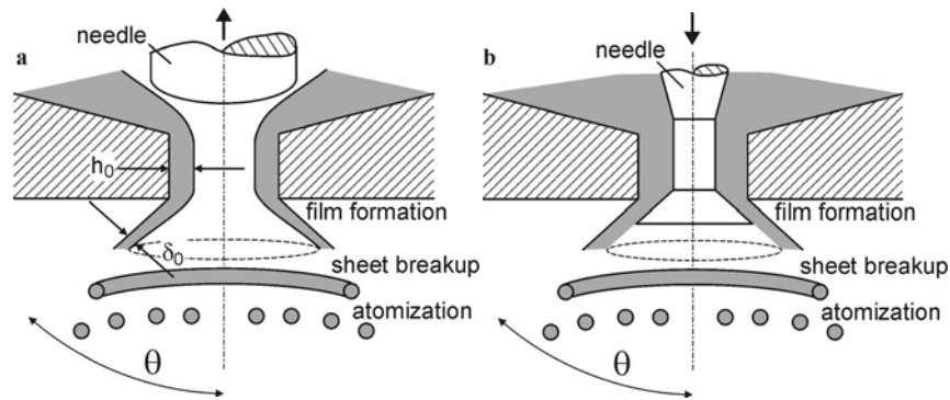
Fig. 4.17. a Inwardly opening pressure-swirl atomizer, b outwardly opening nozzle
