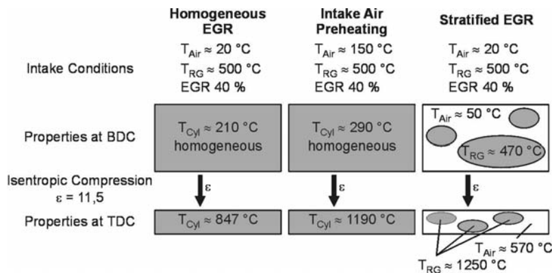
Fig. 6.44. CAI combustion (gasoline): influence of time-temperature history and homogeneity on the ignitability of the mixture [101]
