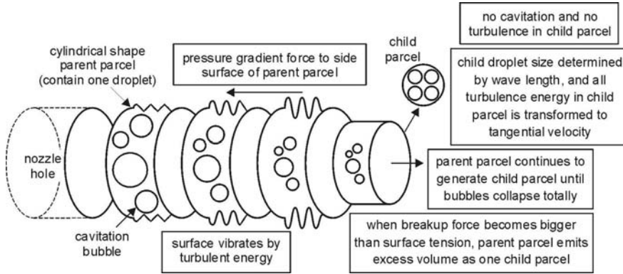
Fig. 4.9 Primary break-up model of Nishimura and Assanis [91]
