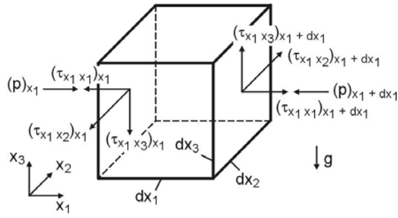
Fig. 3.7. Normal and shear stresses
