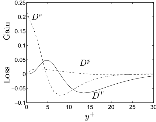
Figure 4.3: Flow between two parallel plates. Direct numerical simulations [21]. Re = U_C \delta / \nu = 7890 . u_*/U_C = 0.050 . Energy balance in k equation. Turbulent diffusion by velocity triple correlations D^T , Turbulent diffusion by pressure D^p , and viscous diffusion D^\nu . All terms have been scaled with u_*^4/\nu .
