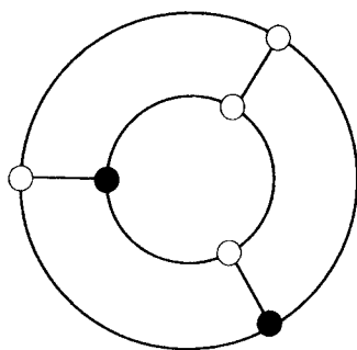
Figure 9-2 A simple binary network.
