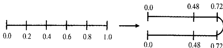
Figure 6-6 The logistic mapping, or "baker transformation."
