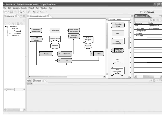
Figure 8: Planned K-Modeler integrated in Eclipse
