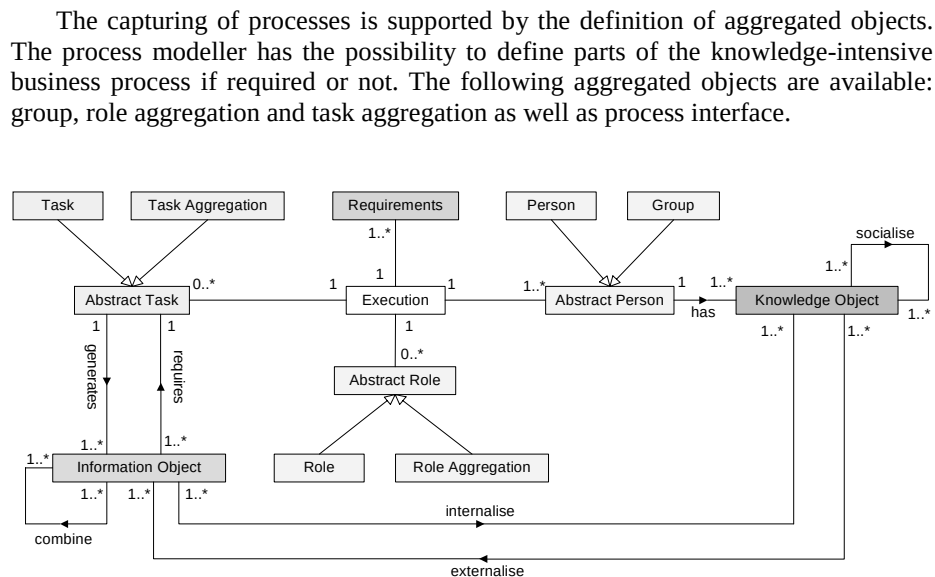
Figure 3: Objects of the KMDL Data Model and their Relations
